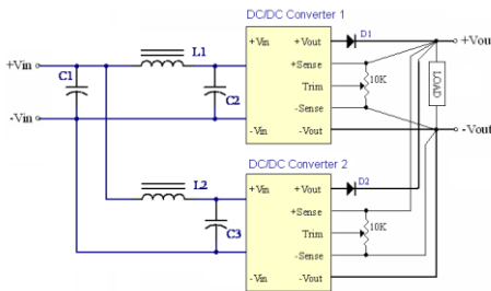
Simple Redundant Operation Connect Circuit L1, L2: 1.0µH C1, C2, C3: 68µF/200V ESR<0.7Ω
