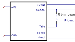
Trim-down Voltage Setup
